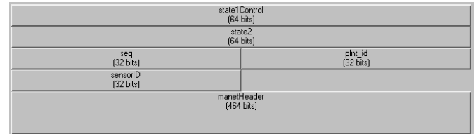
Fig. 7. Simulated/real time packet format for state/control.
