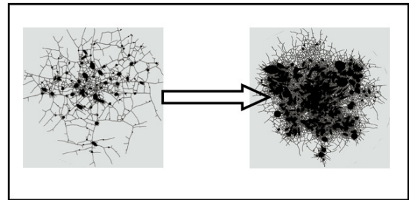
Fig. 4. Increased growth in colonial hydroid stimulated by vitamin C, illustrating redox control of biological tubular networks (Images courtesy Neil Blackstone).
