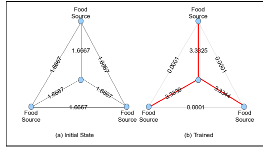
Fig. 6. Simulation of Nakagaki's experimental arrangement (three food sources). In (a), initial vein radii are shown (in arbitrary units). Diagram (b) shows results from a population of 400 virtual ants modeling the flow and resultant signaling over 800 time steps.
