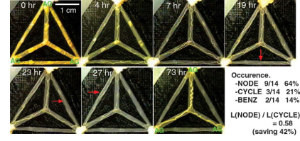
Fig. 5. Triangular model system for experimental investigation of maze traversal, with multiple food sources, by Physarum (Courtesy Toshi Nakagaki).
