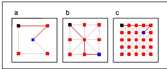
Fig. 7. Simulation of graph traversal by individual virtual ants in the Physarum algorithm, with a single source and destination. Image (a) has five incompletely connected nodes, image (b) nine fully connected nodes and image (c) has 25 fully connected nodes. The resulting path is indicated by the width of the connections.
