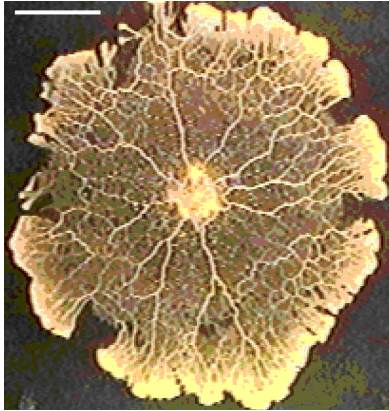
Fig. 2. The structure of Physarum . Dendritic veins radiate from the centre, diverging and bifurcating, to follow the shape and movement of the organism. The graphic distance bar has a length of 1 cm. (Courtesy Toshi Nakagaki).
