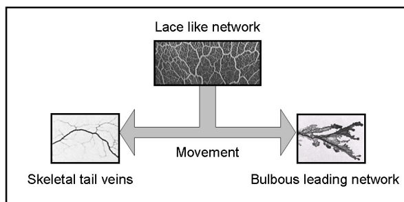
Fig. 3. Movement can induce a leading “bulbous” network, with trailing sparse veins that include relatively large vessels
